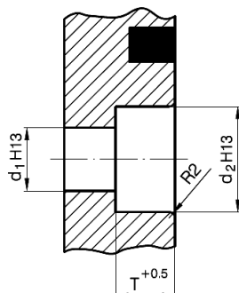
Detail Z
